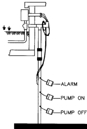
Three Float Demand Switch Bar
