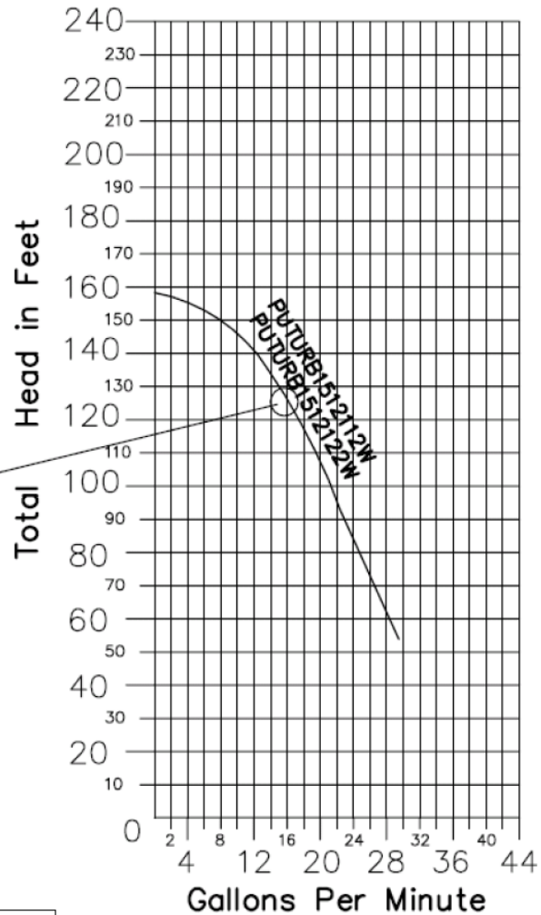
DESIGNERS GUIDE PUMP CURVE DRIP DISPERSAL SYSTEM
