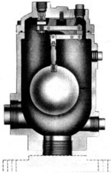
Screwed End Inlet Shown (Flushing Attachments Not Shown)
